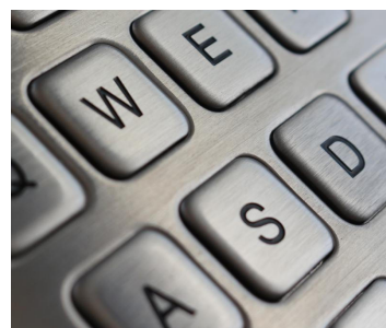
Short stroke with flat keys optional K-TEK-B340KP-FN-DWP
