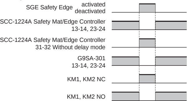
Timing Chart
