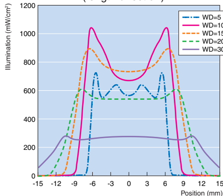
Line beam lens ZUV-L15L Illumination profile (length direction)
