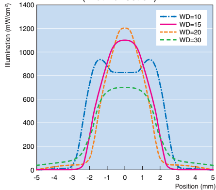
Line beam lens ZUV-L12L Illumination profile (width direction)
